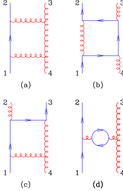
Figure 1. Sample diagrams contributing to the primitive amplitudes (a) A_4^L(\phi, 1_{\bar{q}}, 2_q, 3_g, 4_g) , (b) A_4^R(\phi, 1_{\bar{q}}, 2_q, 3_g, 4_g) , (c) A_4^L(\phi, 1_{\bar{q}}, 2_g, 3_q, 4_g) , and (d) A_4^f(\phi, 1_{\bar{q}}, 2_q, 3_g, 4_g) . The \phi field can attach to any gluon line in the diagram.
